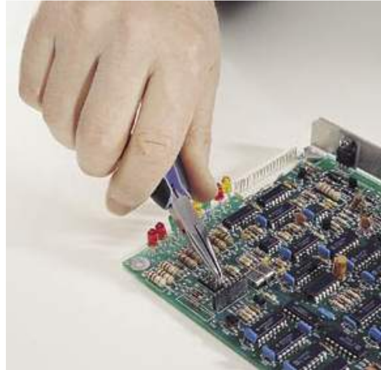
Bent nose Rx7892 allows operator to use an over-hand grip and side access to connector pin and can provide visibility advantages in other applications as well. See page 47 for more on Rx7892.
